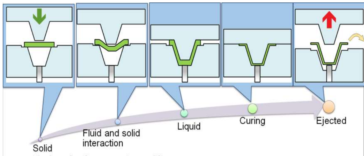
Figure 1: The compression molding process
