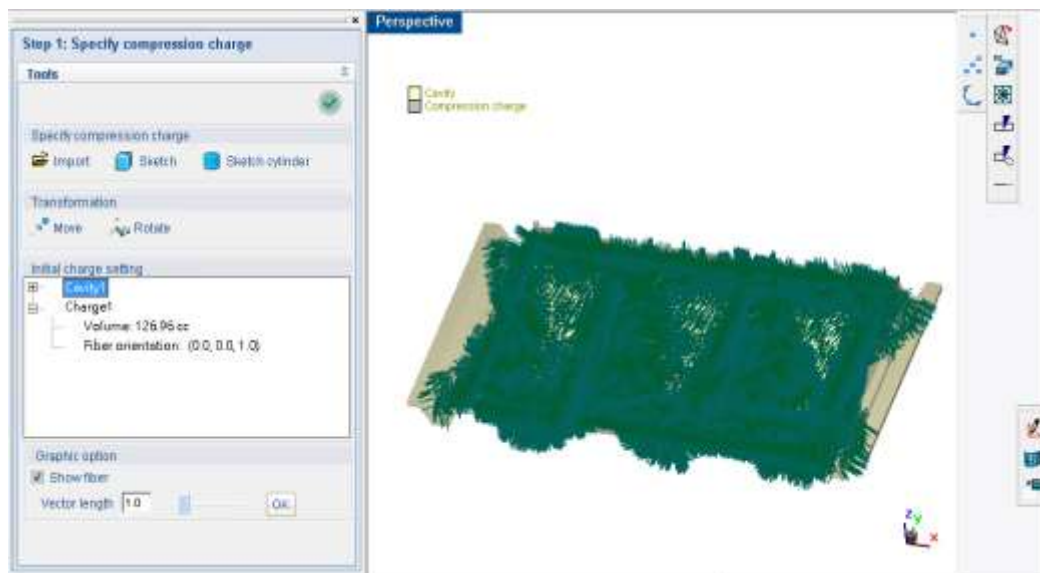
Figure 6. The setting of initial charge shape and initial fiber orientation in Moldex3D
