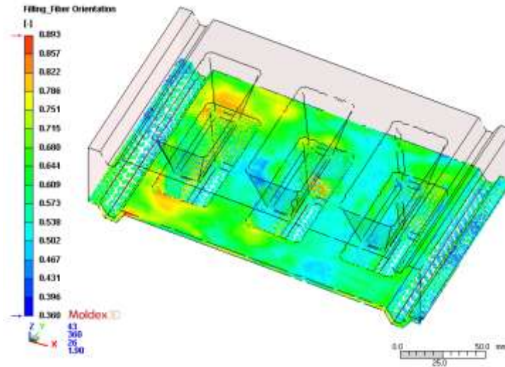
Figure 9. Fiber orientation at EOF
