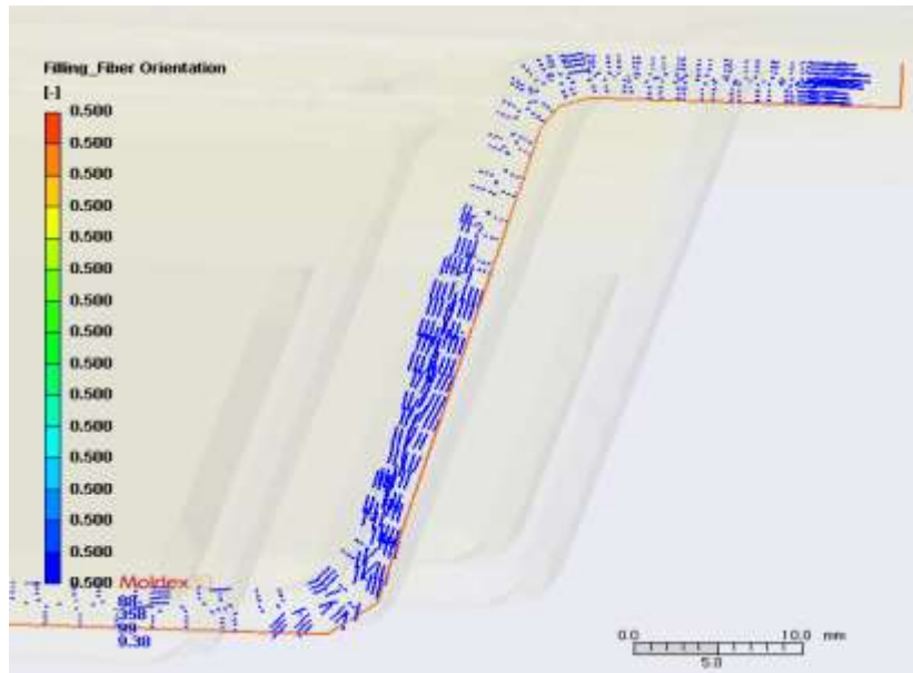
Figure 7. Initial fiber orientation in Moldex3D
