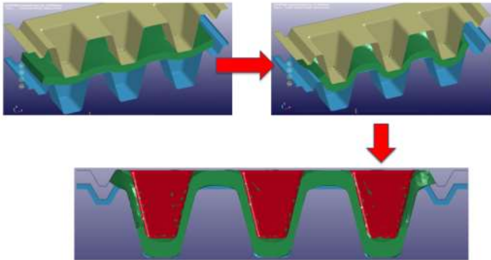
Figure 4. The deformation of the cross-section of the model during forming analysis
