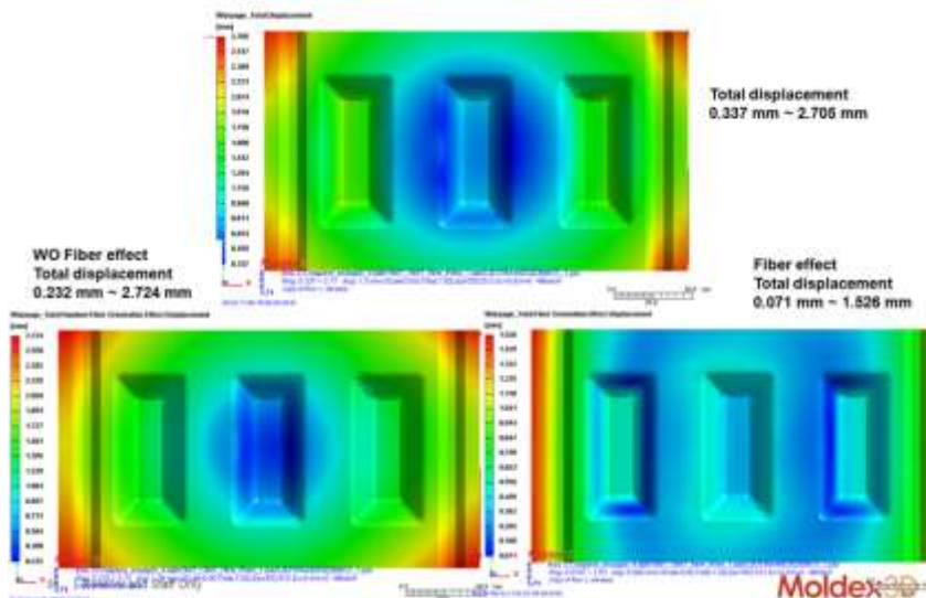
Figure 10. Warpage behavior
